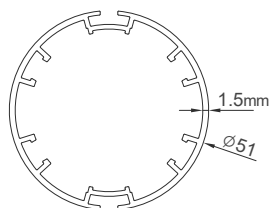
ATD51鋁管 #09503E051
